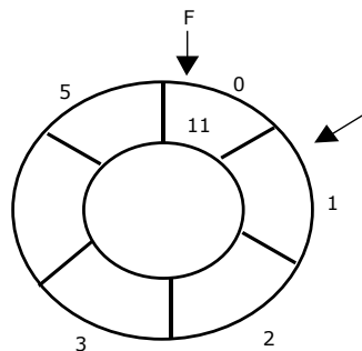
Circular Queue
